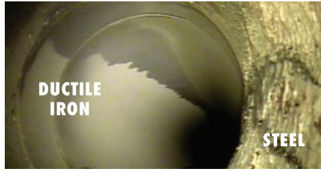
CONTAMINATED STEEL PIPE AFTER 14 YEARS OF SERVICE
